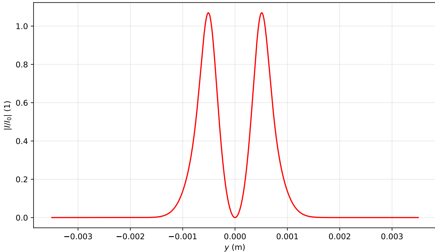
Intensity profile I(x=0, y, z=0.398)/I_0 , P_{in}=5.0P_{cr} , artificial time
